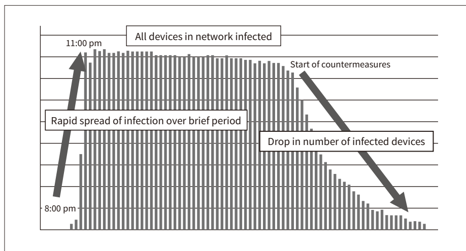
Figure 1 — WannaCry Infection Rate
