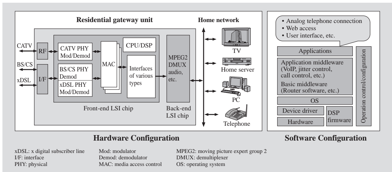
Fig. 3— Internal Configuration of Residential Gateway.
