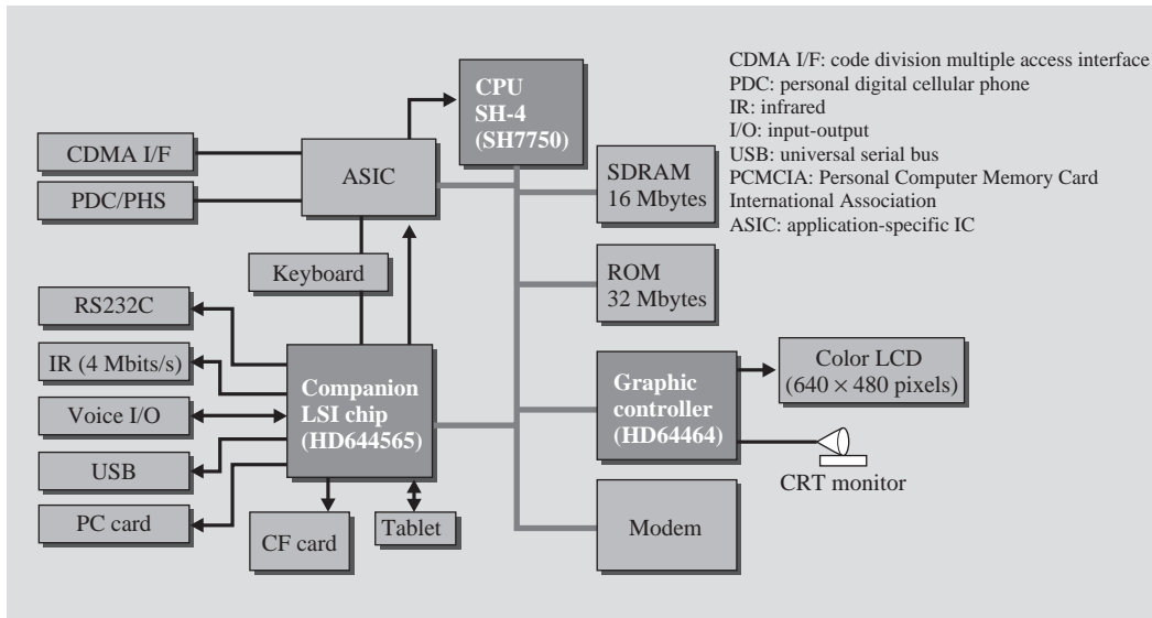
Fig. 6— Hardware Configuration of Handheld PC. Block diagram of HPW-600JC handheld PC. The PC has an SH7750 SuperH RISC engine, a companion LSI chip (HD64465) with peripheral functions, and a built-in graphic controller (HD64464).
