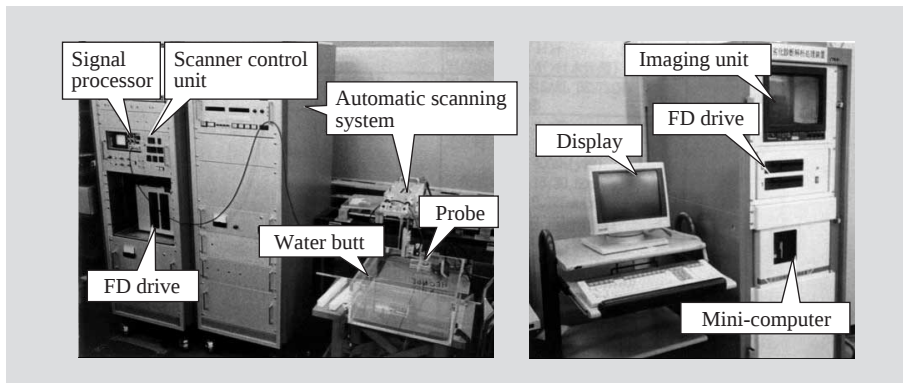
Fig. 4— Ultrasonic Holography System.
