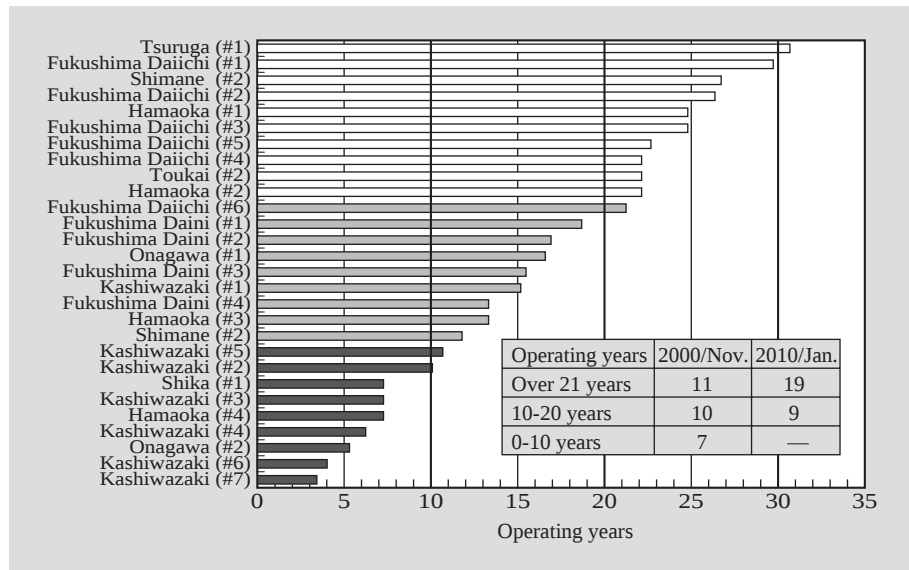
Fig. 1— Number of Operating Years for BWR Power Plants in Japan.
