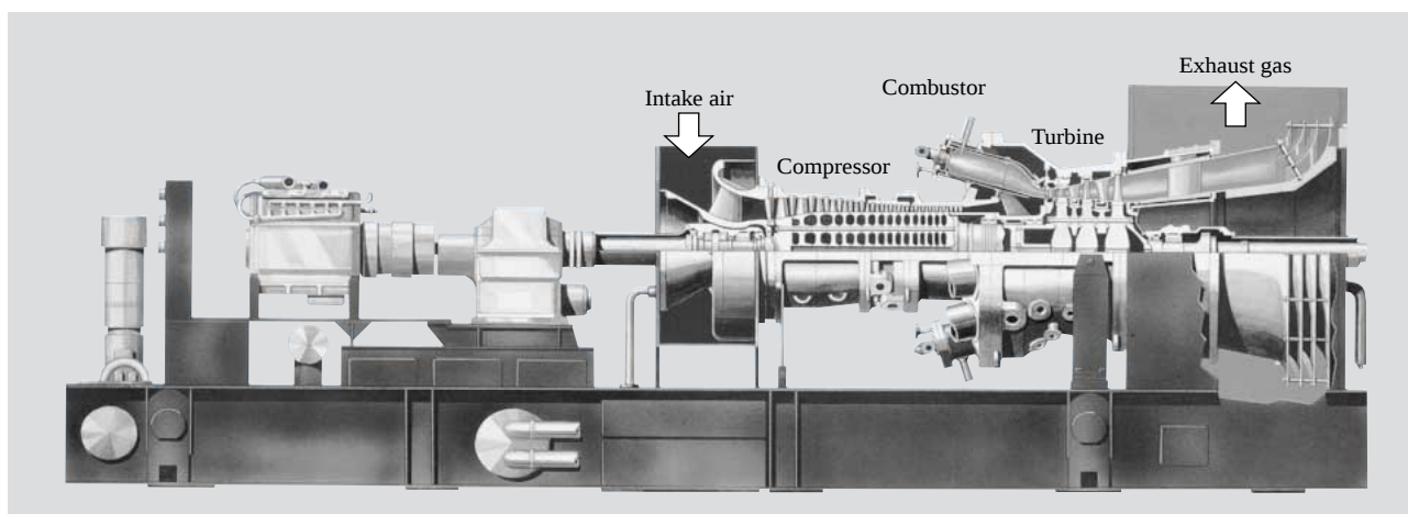
Fig. 2—Cross Section of H-25 Gas Turbine.
