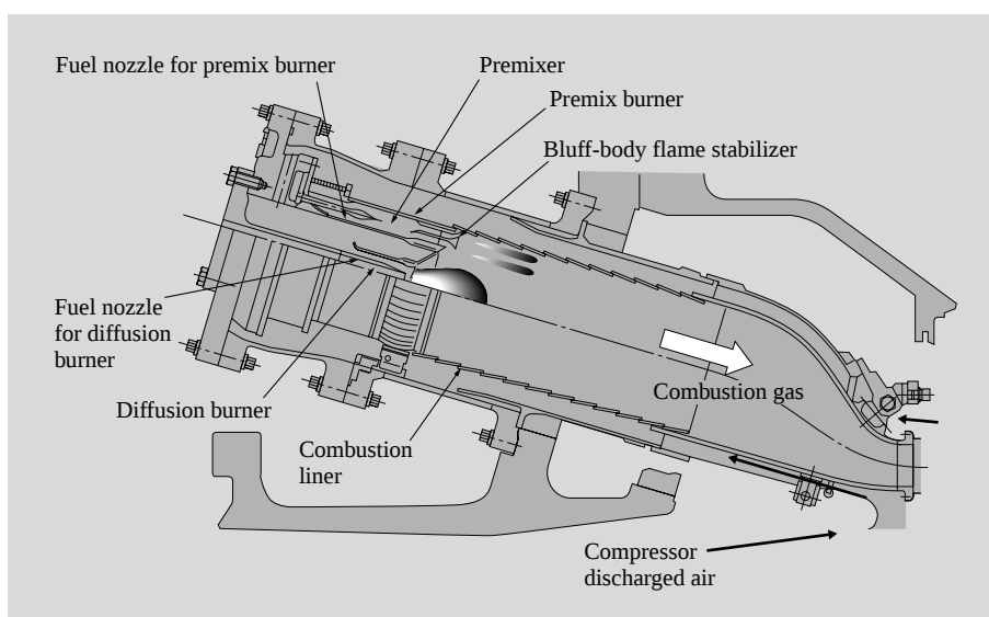
Fig. 3—Structure of Low-NO x Combustor Incorporated in H-25 Gas-turbine Generator.
