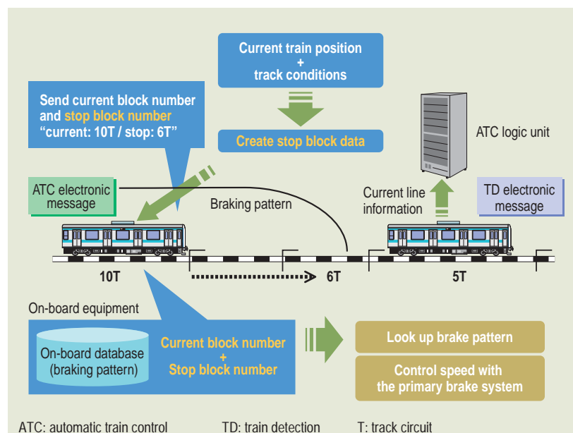
Digital ATC system
