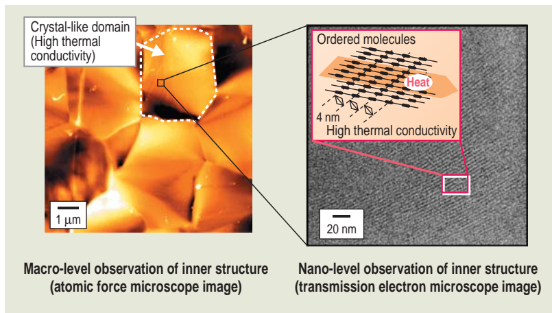
Inner structure of highly thermally conductive resin
