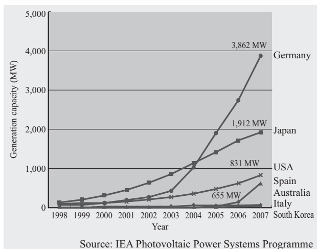
Fig. 2—Cumulative Installed Photovoltaic Power Generation Capacity in Leading Countries.
