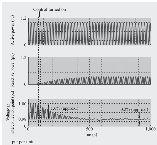
Fig. 5—Effect of Function for Reducing Grid Voltage Fluctuation.
