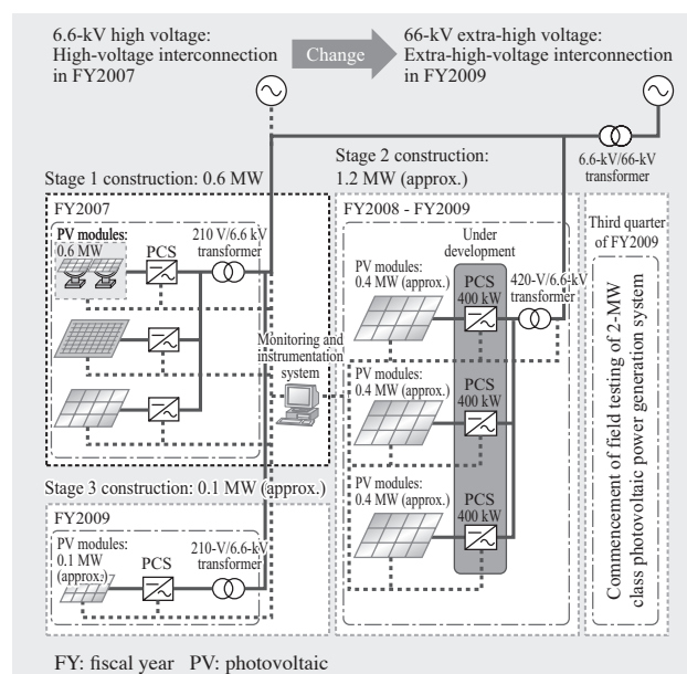
Fig. 7—Overall Configuration of Hokuto Project.
