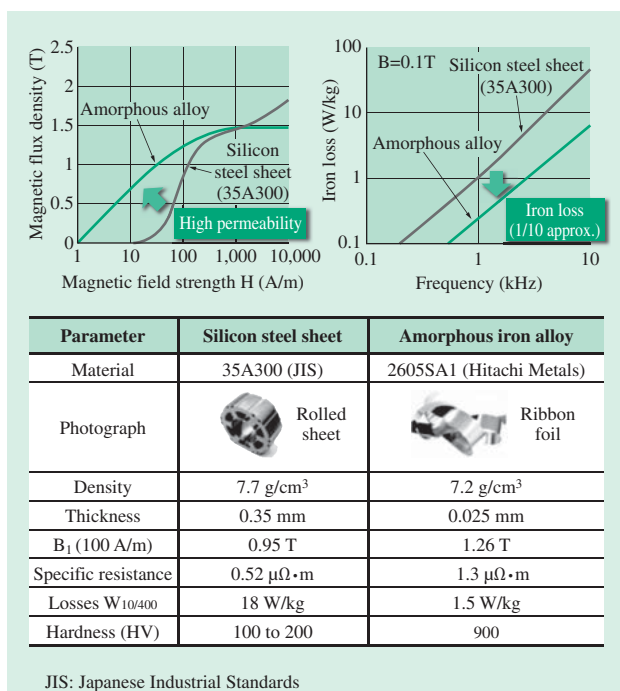
Fig. 2—Properties of Amorphous Iron Alloy.
