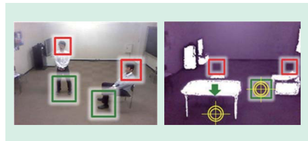
Fig. 9—Detection of People's Feet (Left) and Detection of Air Flow Paths when Heating (Right).
