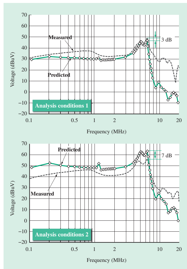
Fig. 6—Comparison of Analysis and Measurement of Radiated Emissions.
