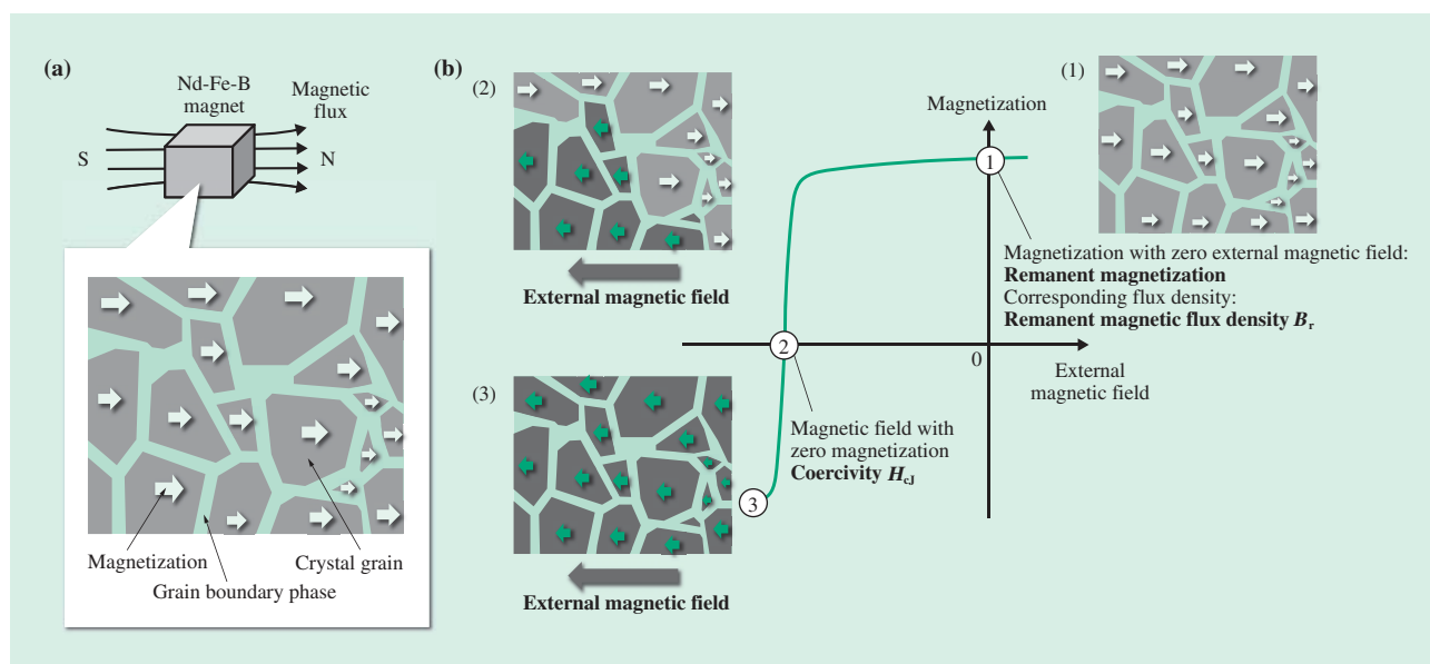
Fig. 2—Schematic Diagrams of Microstructure and Magnetic Properties of Nd-Fe-B Magnets.
