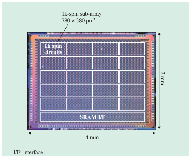
Fig. 5—Ising Chip Photograph.
