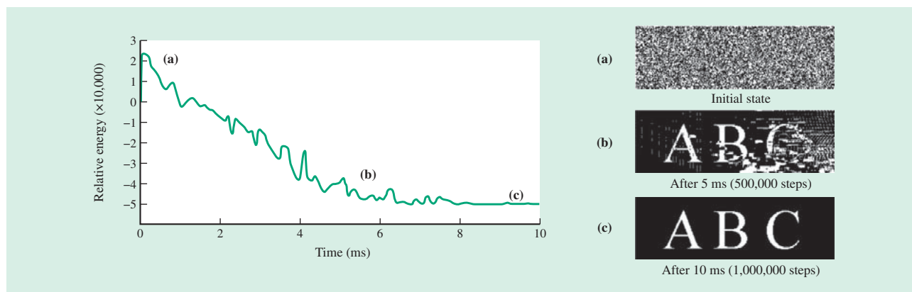
Fig. 8—Changes in Energy and Spin States while Solving a Combinatorial Optimization Problem.
