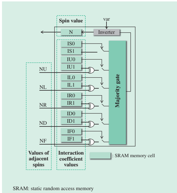
Fig. 3—Spin Circuit for Single Spin.
