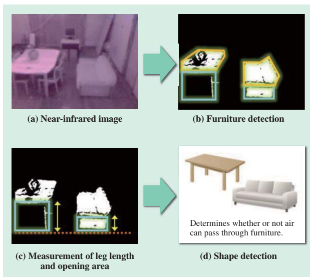
Fig. 7—Furniture Detection Using Near-infrared Images and Image Processing.
