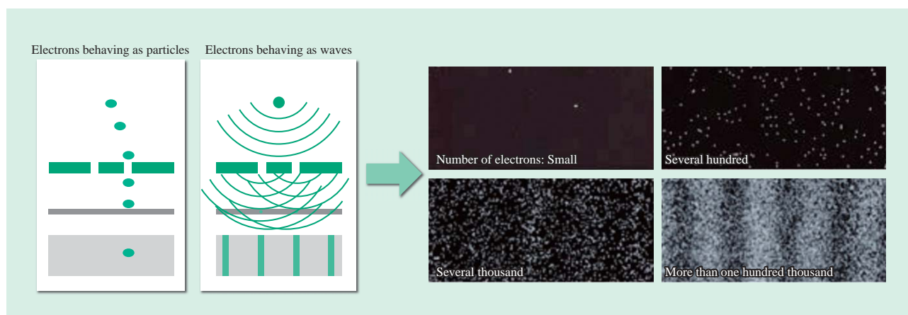
Fig. 4—Electron Double-slit Experiment.
