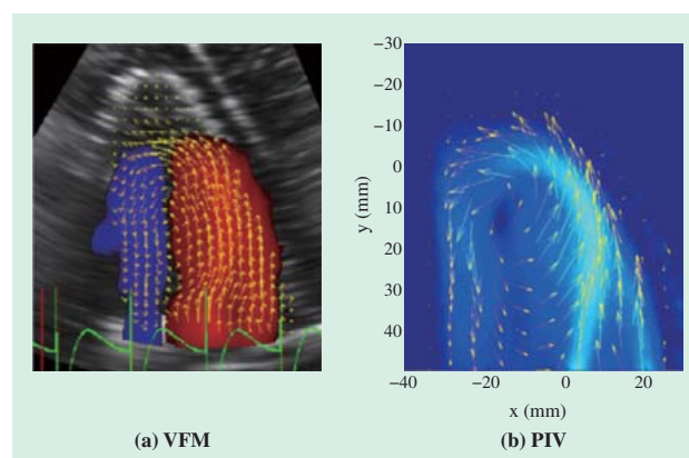
Fig. 5—Comparison of Blood Flow Patterns Obtained Using VFM and PIV.
