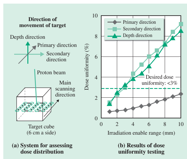
Fig. 7—Results of Dose Distribution Testing.
