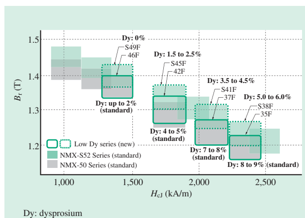
Fig. 11—Characteristics Map of Dy-free Nd-Fe-B Magnet (4) .
