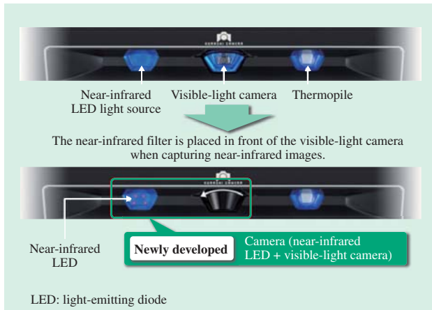
Fig. 6—Multi-monitoring System Components.
