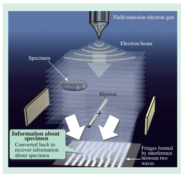
Fig. 1—Principle of Holography Electron Microscope.
