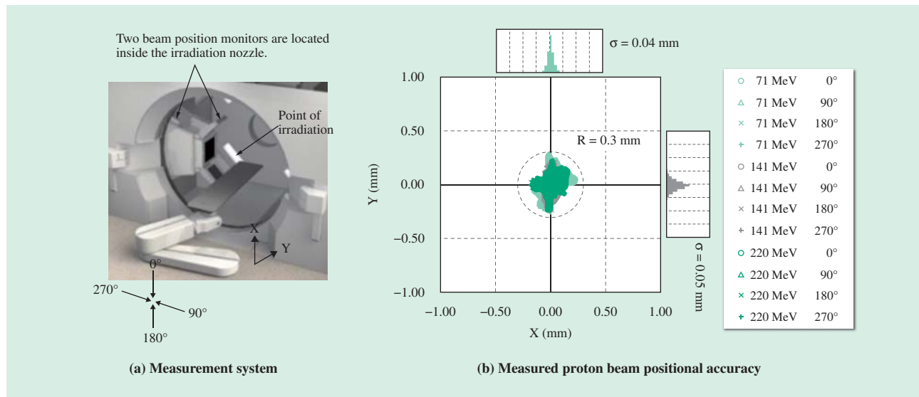
Fig. 8—Proton Beam Irradiation Performance Testing.
