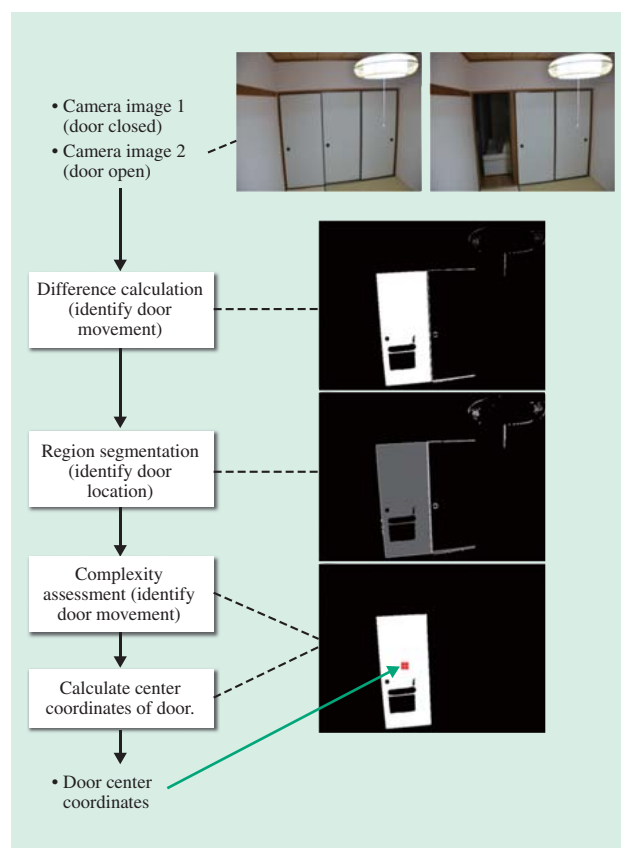
Fig. 2—Sequence of Steps for Door Detection.
