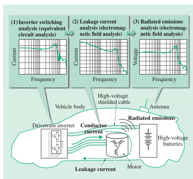
Fig. 3—Vehicle-level Analysis.
