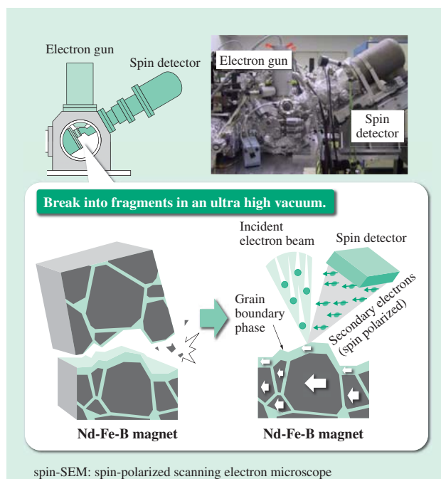
Fig. 6—Magnetization Measurement of Grain Boundary Phase Using Spin-SEM.
