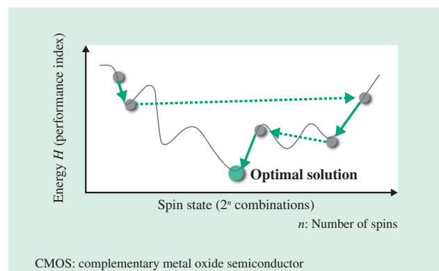
Fig. 4—Ising Model Energy Profile and CMOS Annealing.
