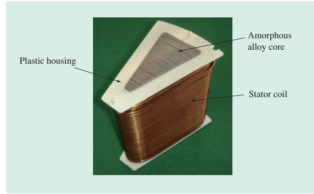
Fig. 9—Design of Amorphous Alloy Core.
