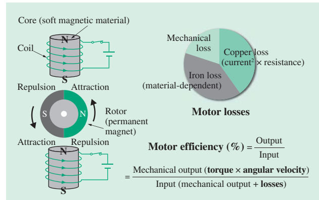
Fig. 3—Principle of Operation of Permanent Magnet Motor, Breakdown of Losses, and Definition of Motor Efficiency.
