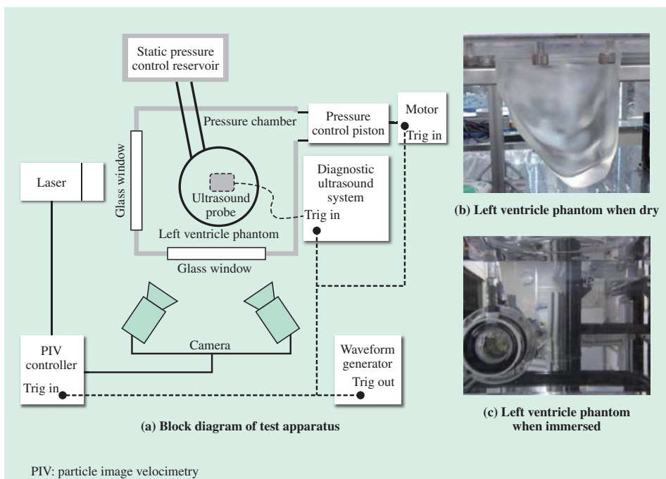
Fig. 4—Overview of Test Apparatus.
