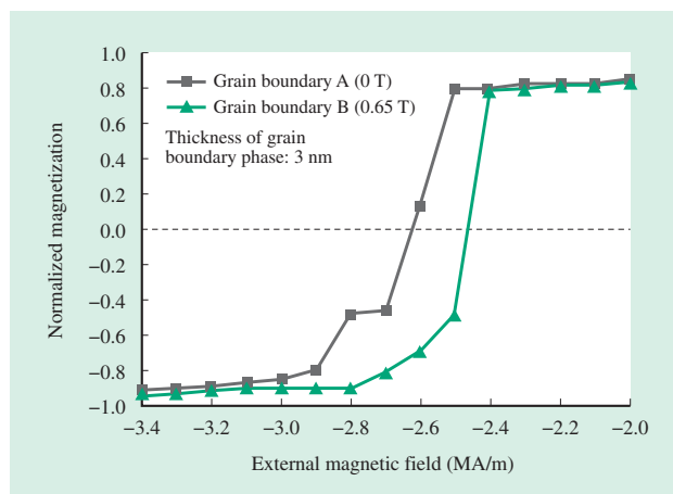
Fig. 10—Results of Calculating Magnetization Curve Using Four-grain Model.
