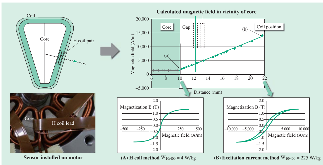
Fig. 7—Overview of Measurement Method for Determining Magnetic Field Applied to Core.
