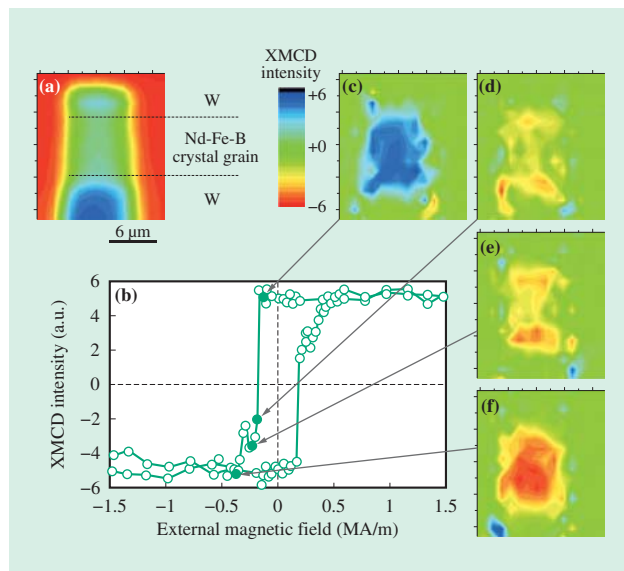
Fig. 5—Magnetization Map during Magnetization Reversal in Microscopic Nd-Fe-B Crystal Grain.
