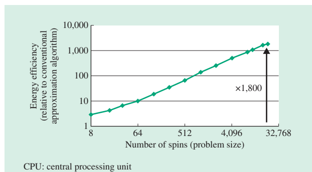
Fig. 9—Energy Efficiency of Solving Randomly Generated Maximum Cut Problem.
